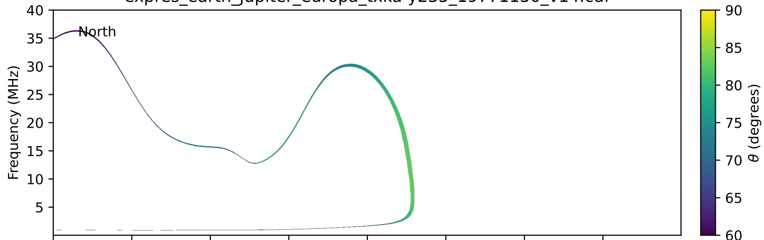
expres_earth_jupiter_europa_txka-y235_19771130_v14.cdf
