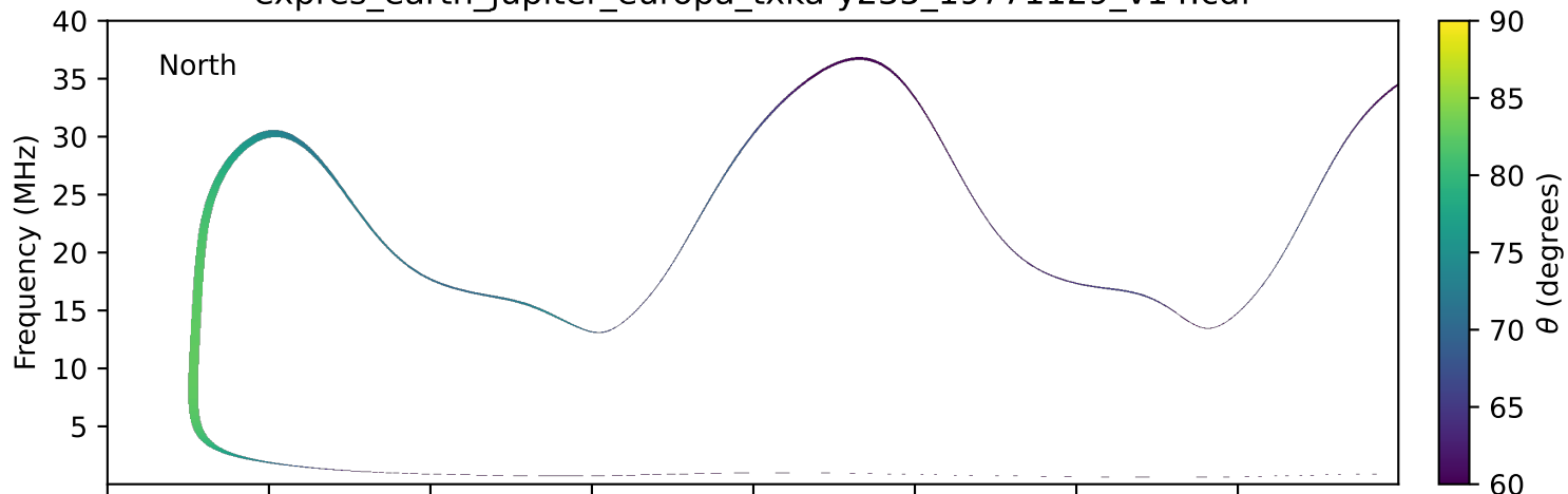
expres_earth_jupiter_europa_txka-y235_19771129_v14.cdf
