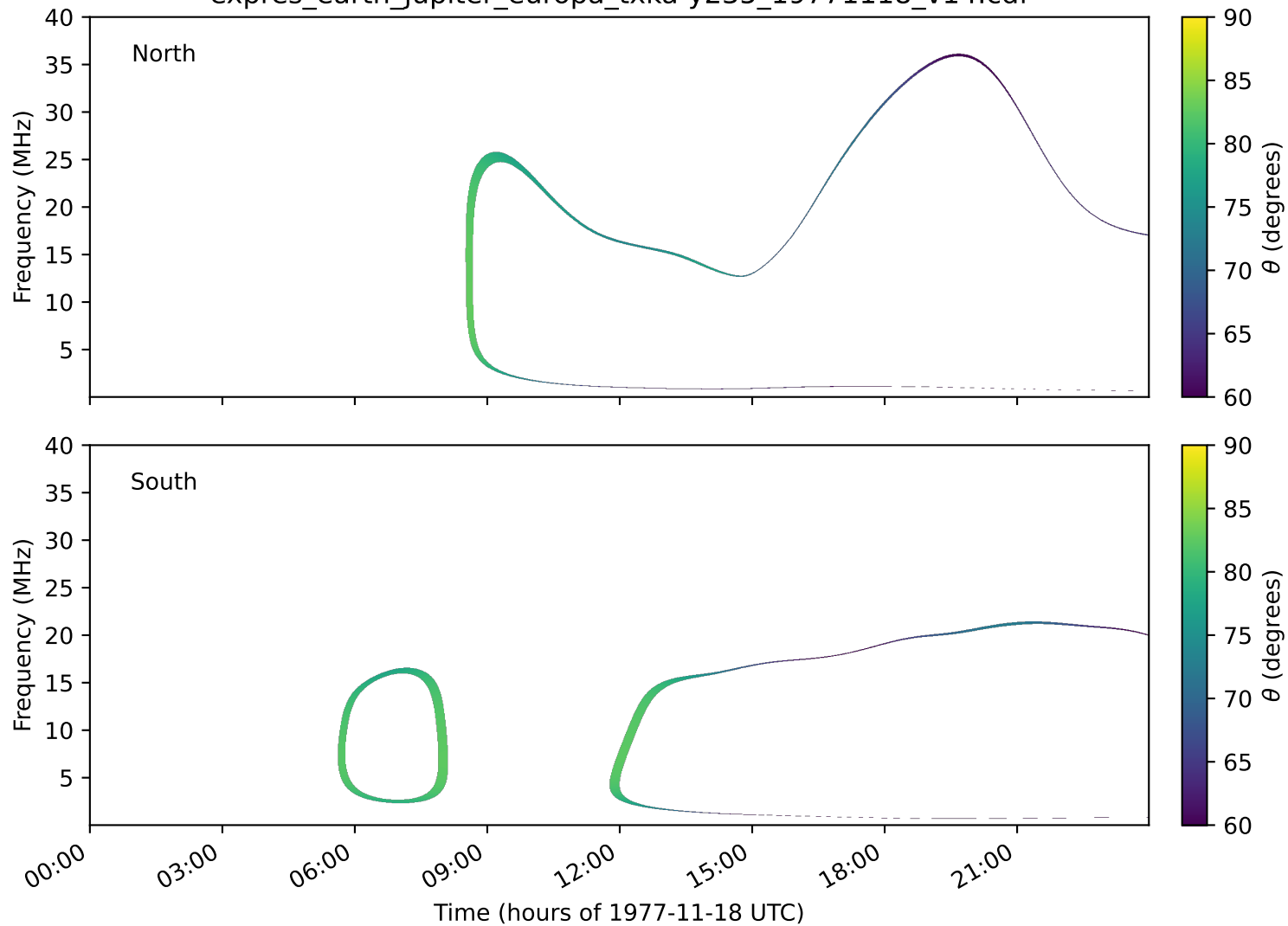
expres_earth_jupiter_europa_txka-y235_19771118_v14.cdf
