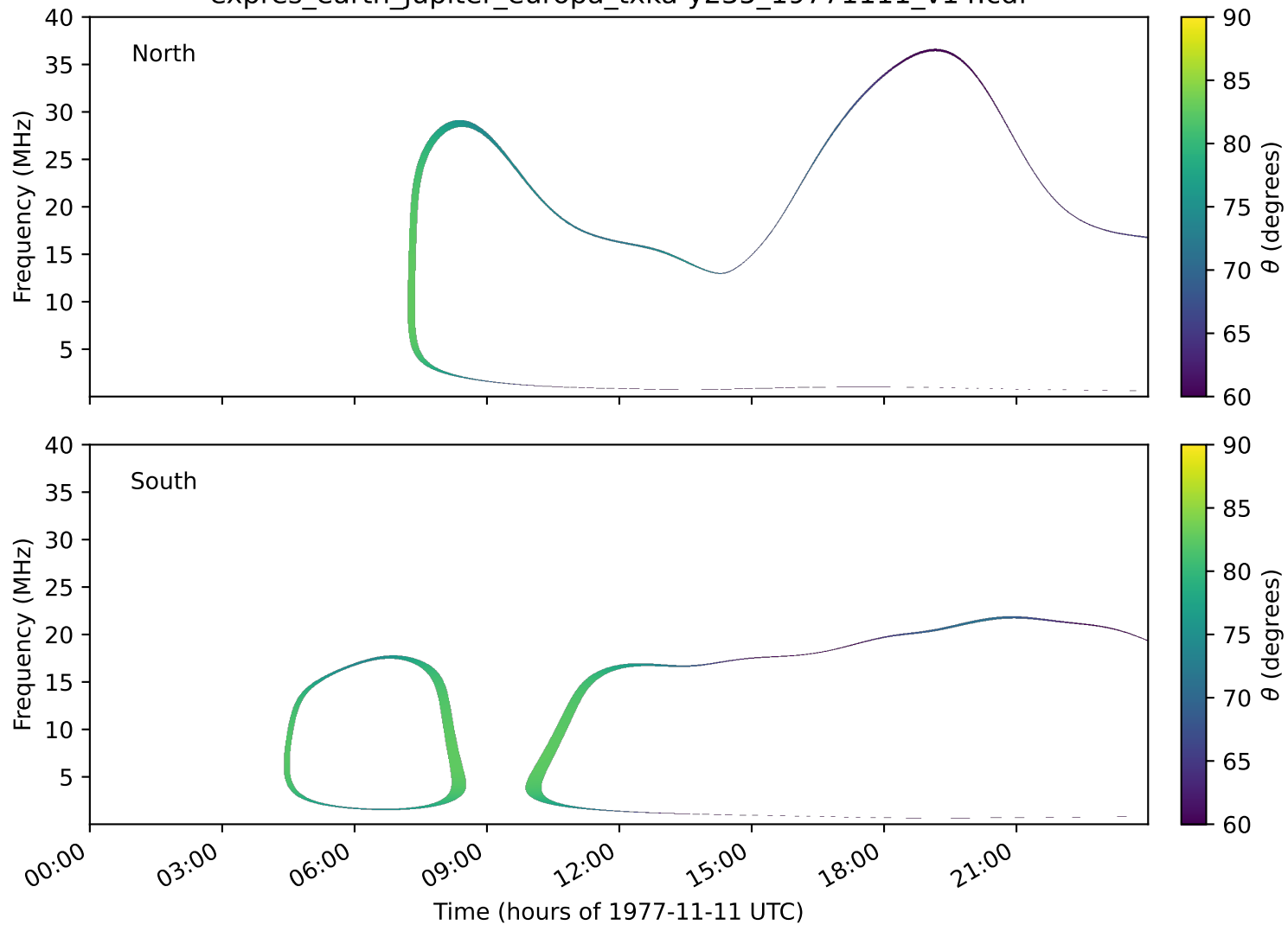
expres_earth_jupiter_europa_txka-y235_19771111_v14.cdf
