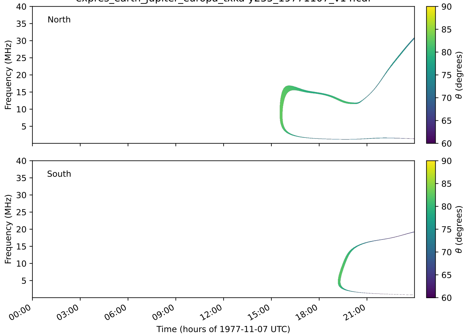
expres_earth_jupiter_europa_txka-y235_19771107_v14.cdf
