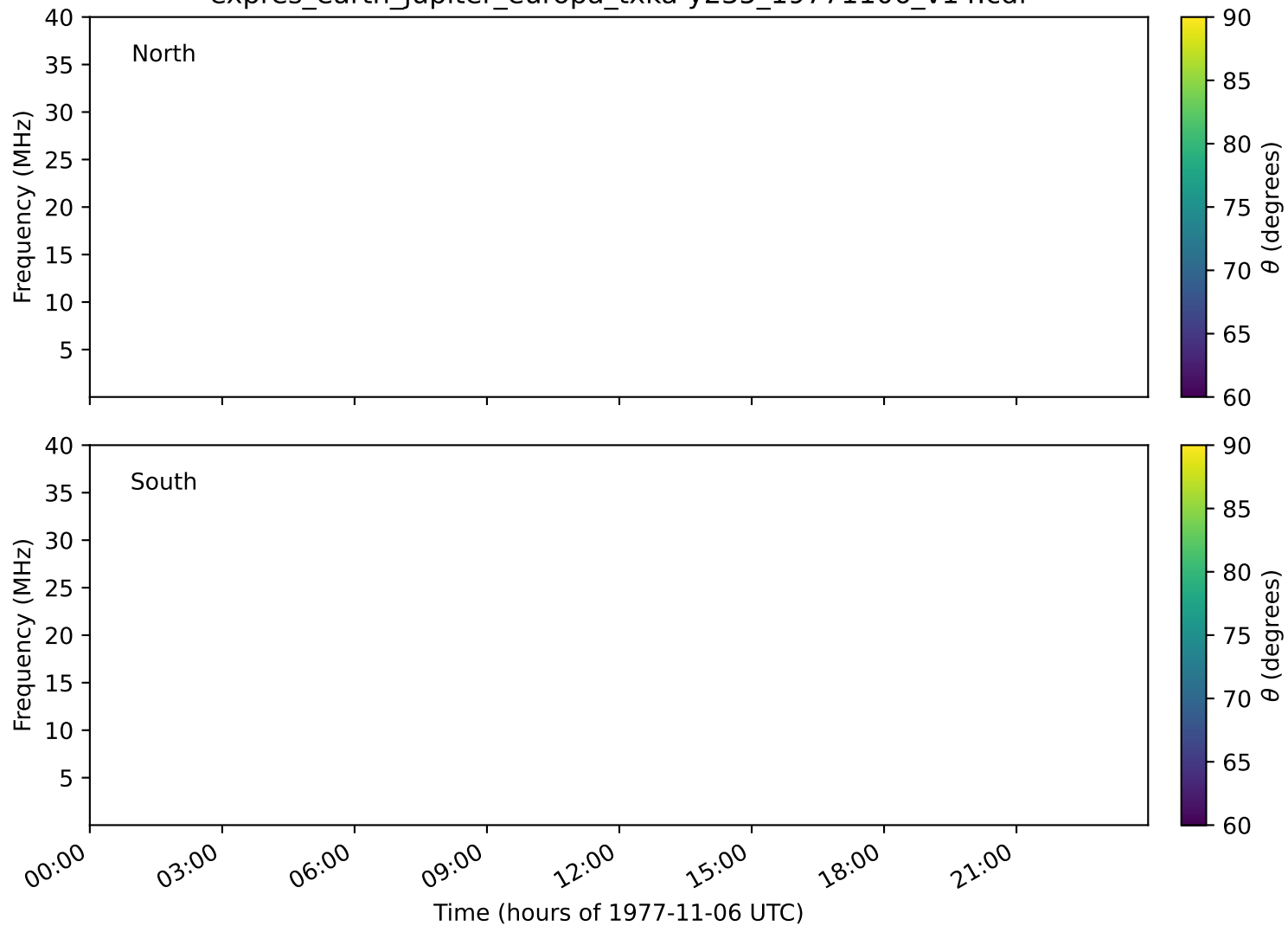
expres_earth_jupiter_europa_txka-y235_19771106_v14.cdf
