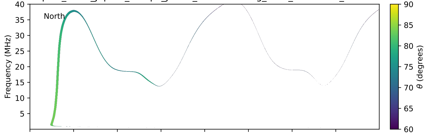
expres_earth_jupiter_europa_jrm33_lossc-wid1deg_3kev_19771129_v11.cdf
