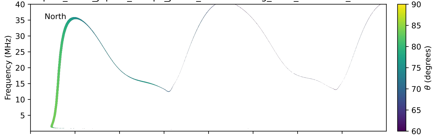
expres_earth_jupiter_europa_jrm09_lossc-wid1deg_3kev_19771129_v11.cdf
