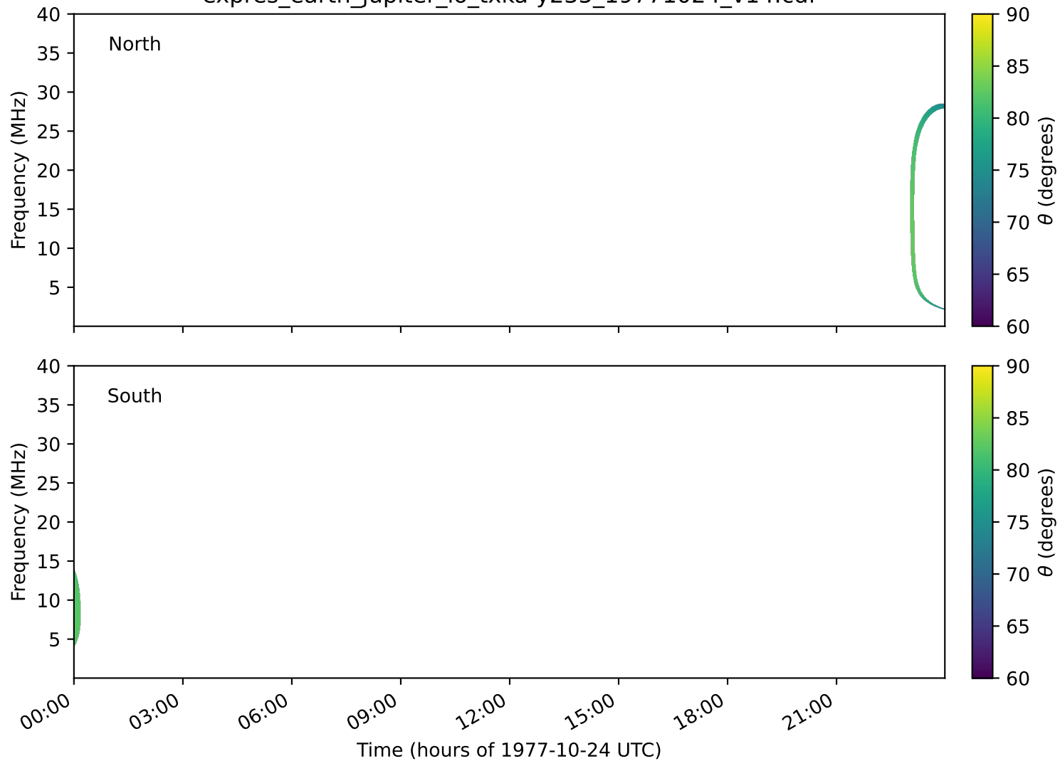
expres_earth_jupiter_io_txka-y235_19771024_v14.cdf
