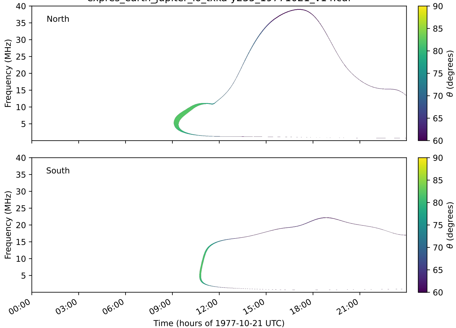
expres_earth_jupiter_io_txka-y235_19771021_v14.cdf
