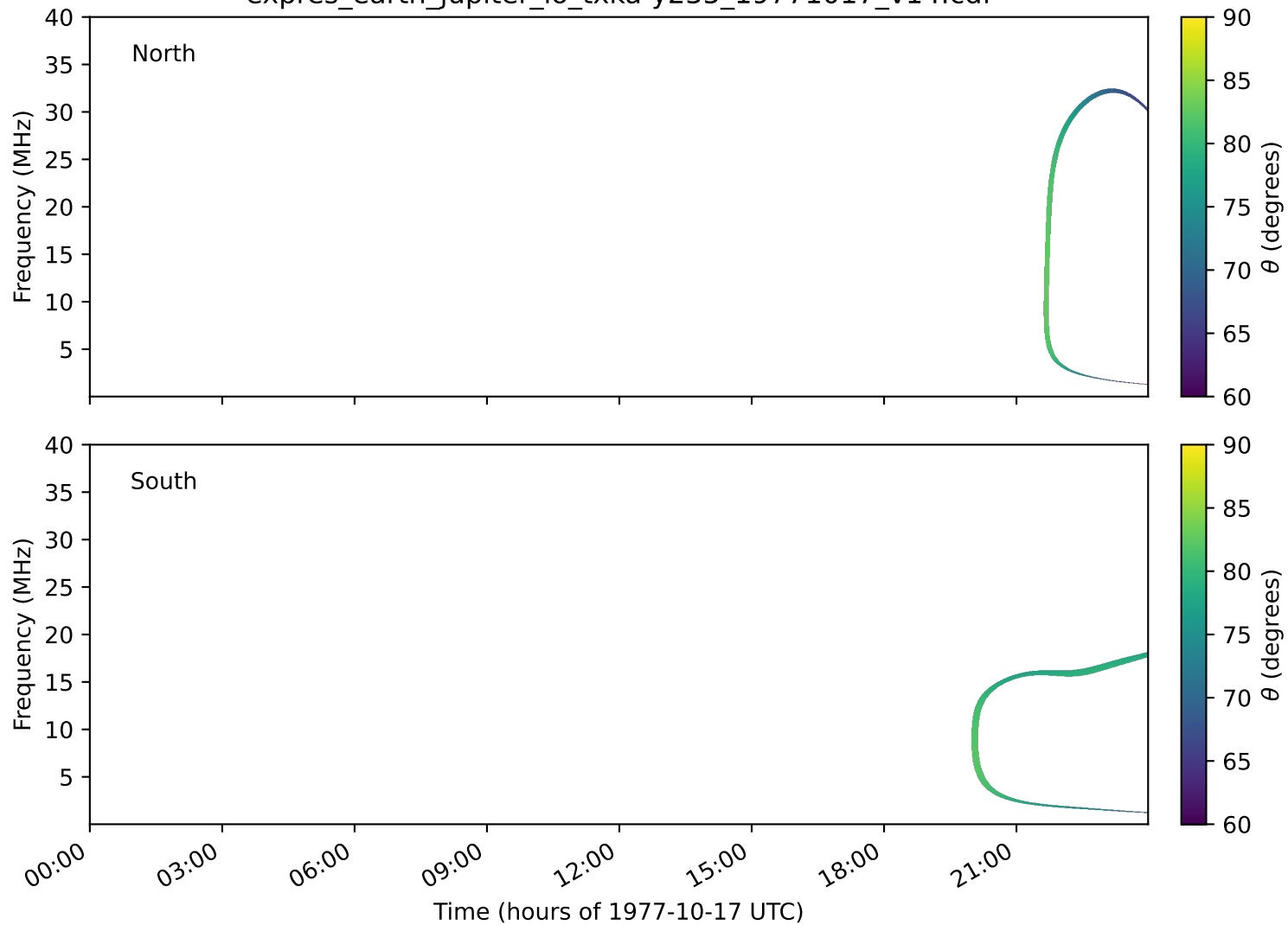
expres_earth_jupiter_io_txka-y235_19771017_v14.cdf
