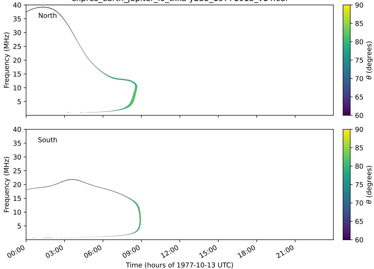
expres_earth_jupiter_io_txka-y235_19771013_v14.cdf
