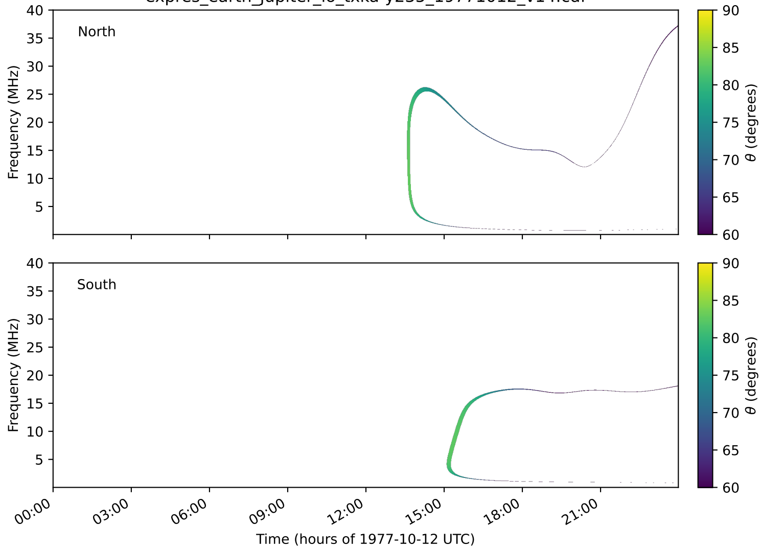
expres_earth_jupiter_io_txka-y235_19771012_v14.cdf
