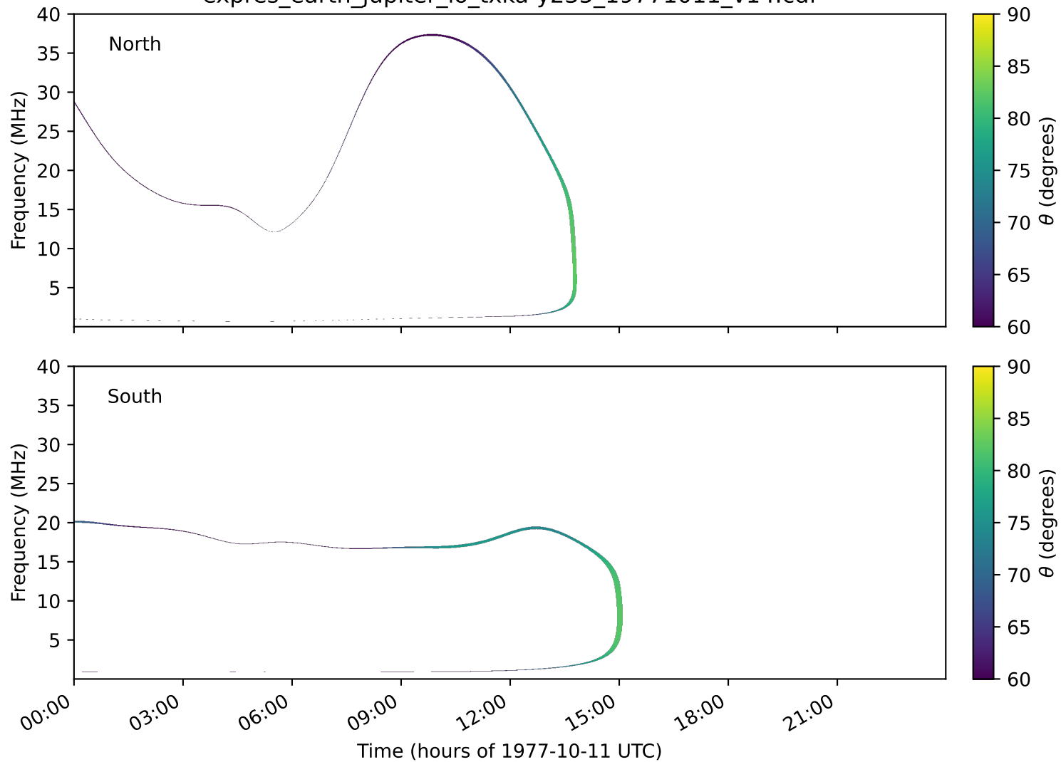
expres_earth_jupiter_io_txka-y235_19771011_v14.cdf
