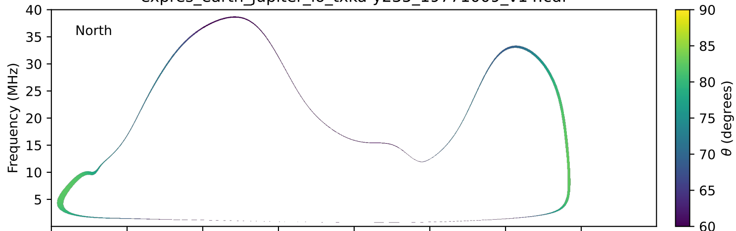
expres_earth_jupiter_io_txka-y235_19771009_v14.cdf
