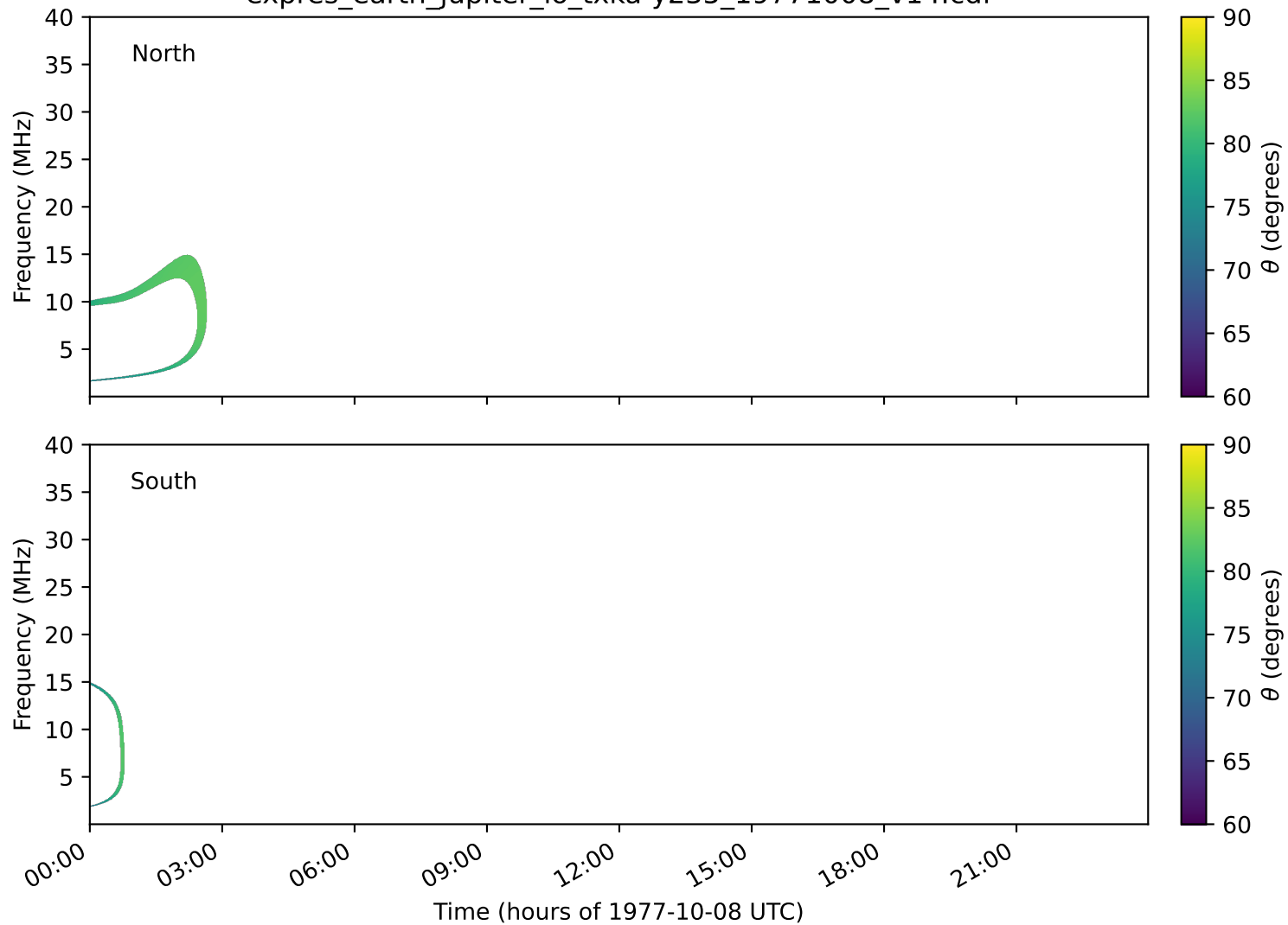
expres_earth_jupiter_io_txka-y235_19771008_v14.cdf
