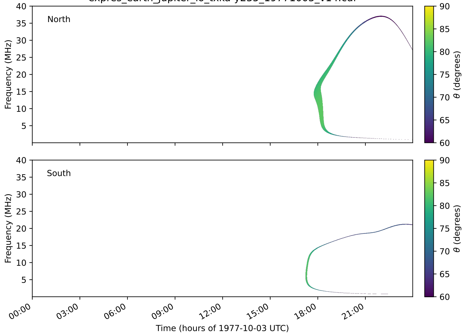
expres_earth_jupiter_io_txka-y235_19771003_v14.cdf
