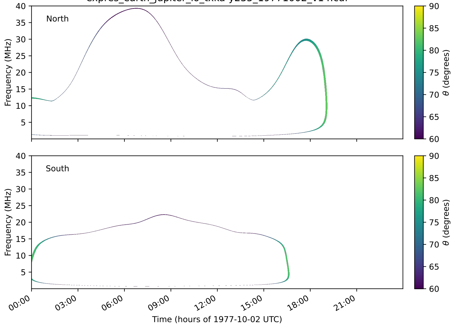
expres_earth_jupiter_io_txka-y235_19771002_v14.cdf
