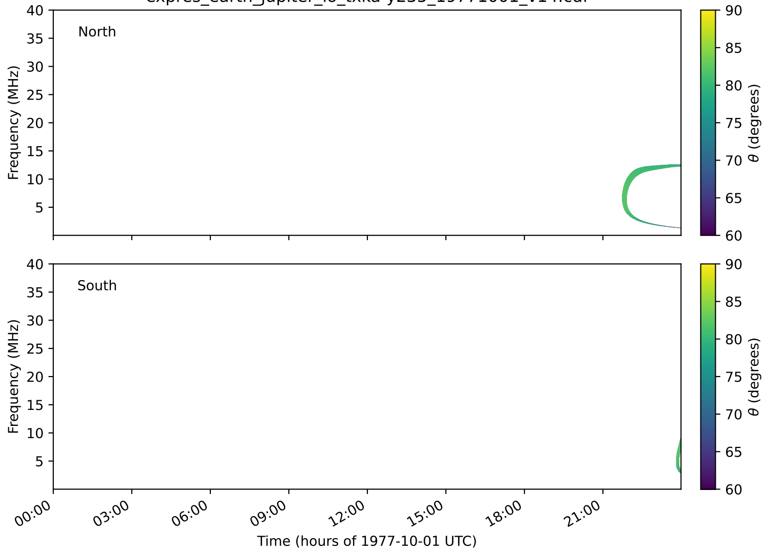
expres_earth_jupiter_io_txka-y235_19771001_v14.cdf
