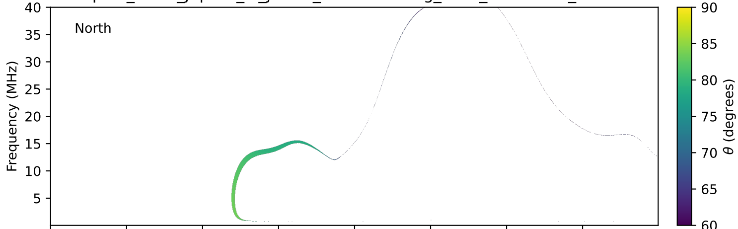
expres_earth_jupiter_io_jrm33_lossc-wid1deg_3kev_19771014_v11.cdf
