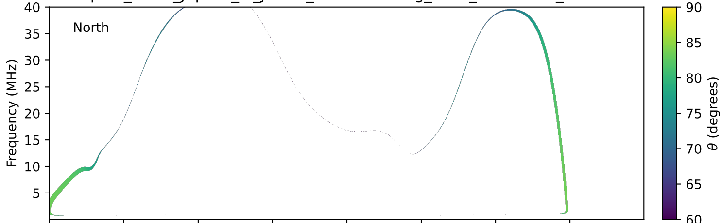
expres_earth_jupiter_io_jrm33_lossc-wid1deg_3kev_19771009_v11.cdf
