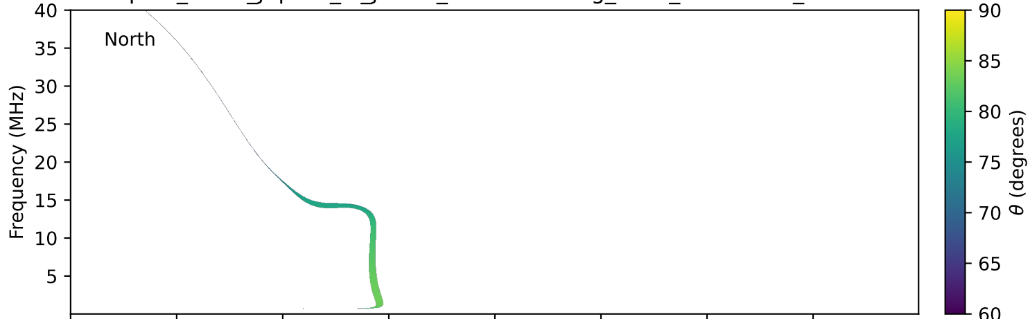
expres_earth_jupiter_io_jrm09_lossc-wid1deg_3kev_19771013_v11.cdf
