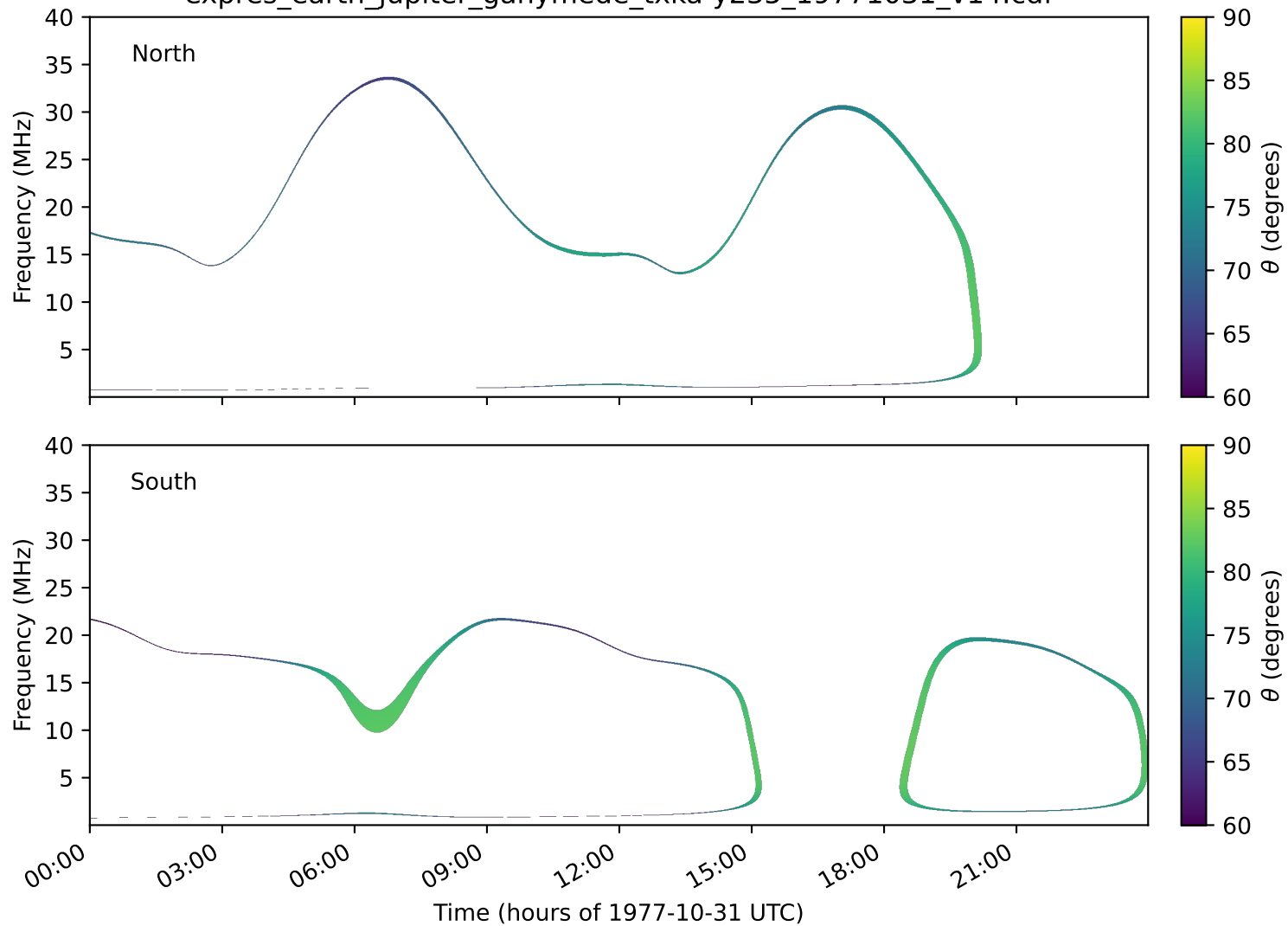
expres_earth_jupiter_ganymede_txka-y235_19771031_v14.cdf
