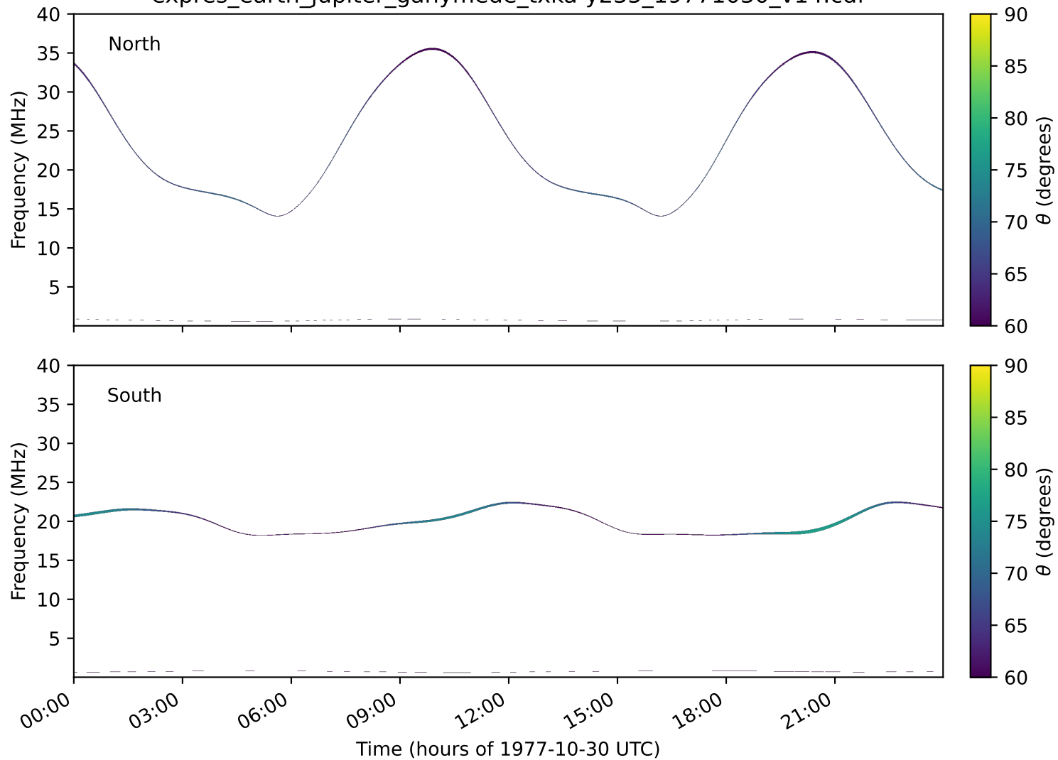
expres_earth_jupiter_ganymede_txka-y235_19771030_v14.cdf
