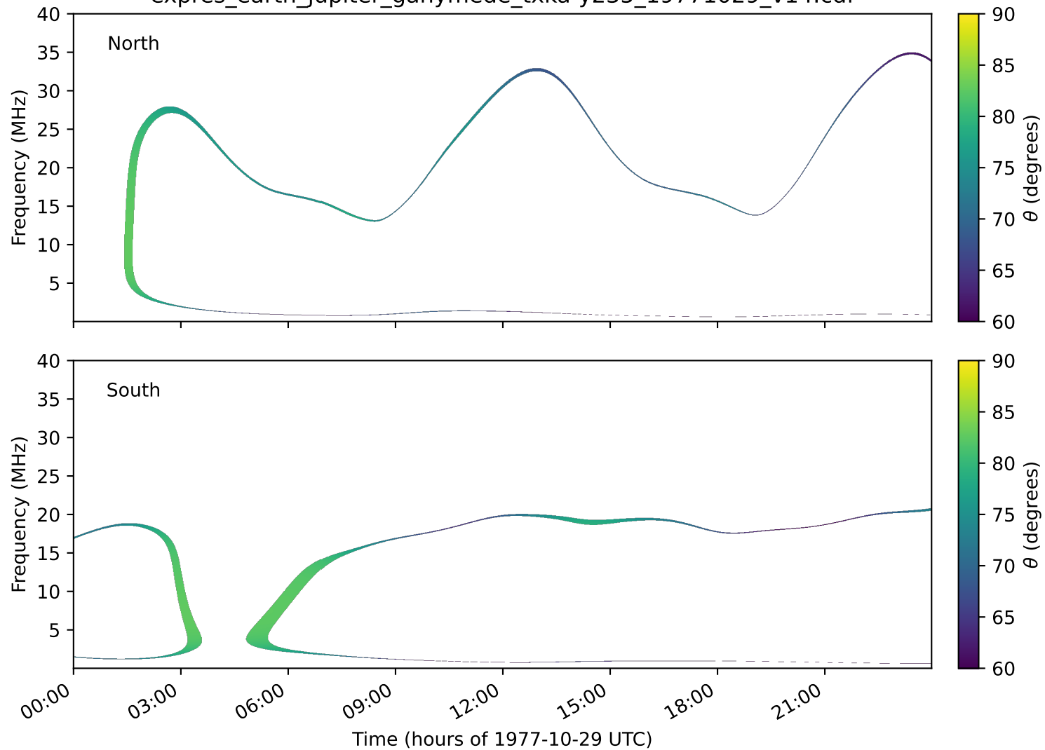
expres_earth_jupiter_ganymede_txka-y235_19771029_v14.cdf
