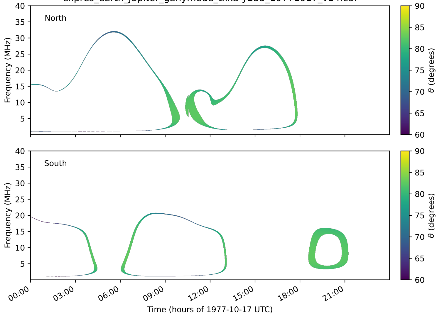
expres_earth_jupiter_ganymede_txka-y235_19771017_v14.cdf
