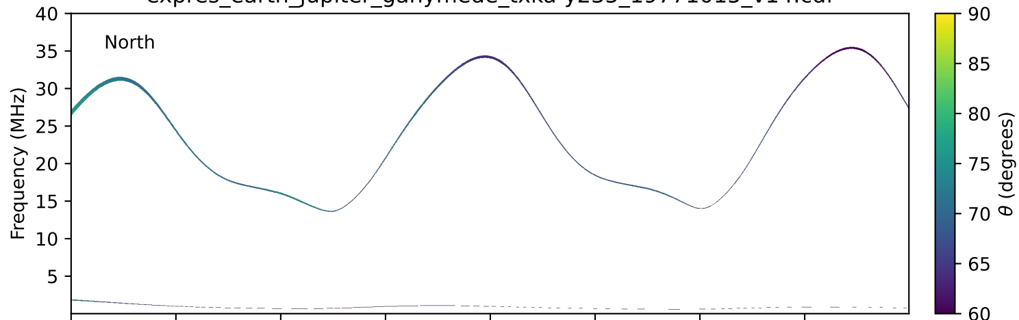
expres_earth_jupiter_ganymede_txka-y235_19771015_v14.cdf
