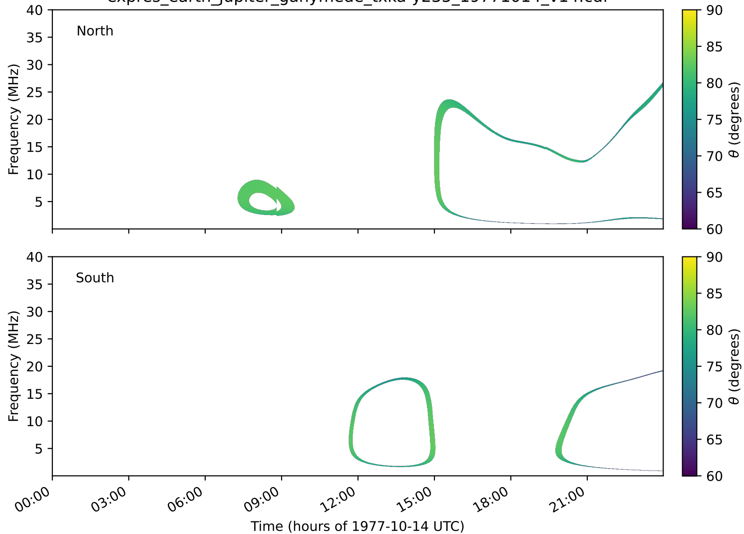
expres_earth_jupiter_ganymede_txka-y235_19771014_v14.cdf
