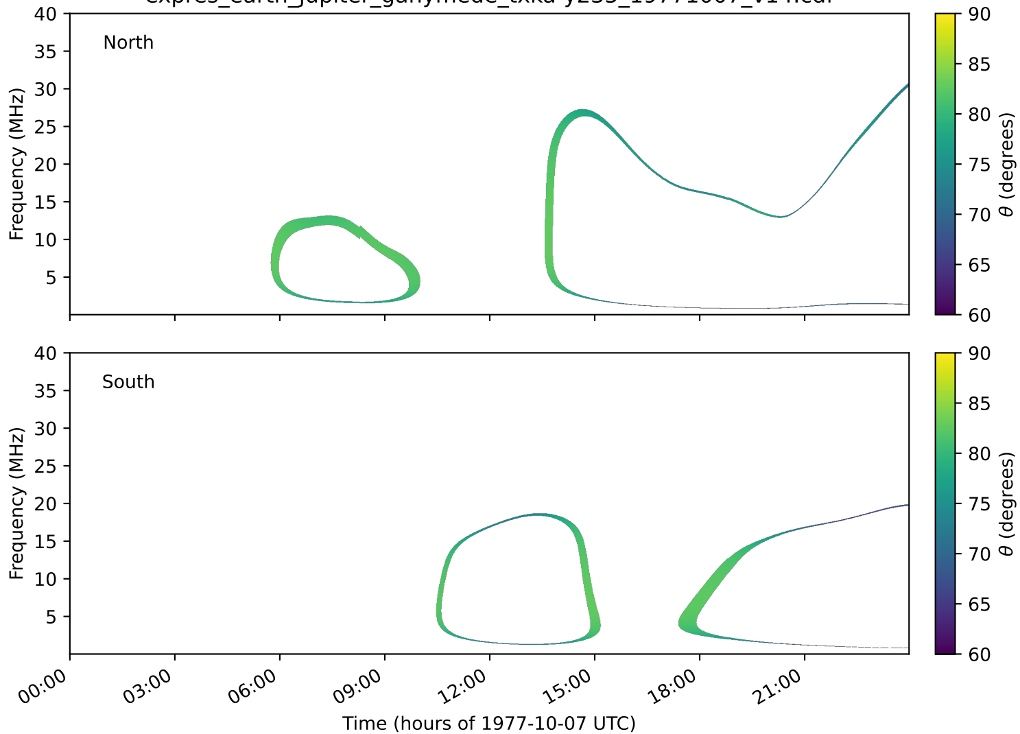
expres_earth_jupiter_ganymede_txka-y235_19771007_v14.cdf
