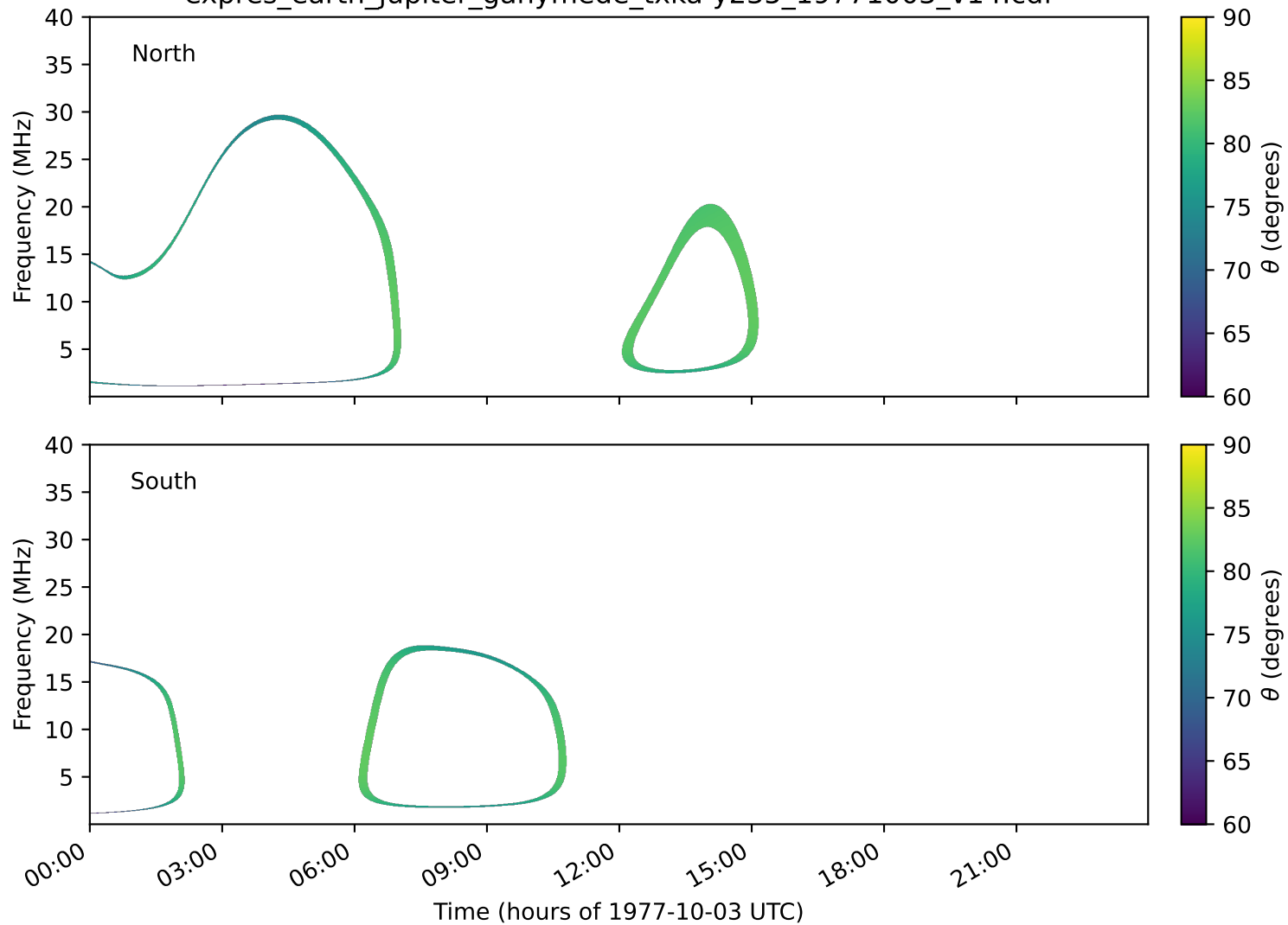
expres_earth_jupiter_ganymede_txka-y235_19771003_v14.cdf
