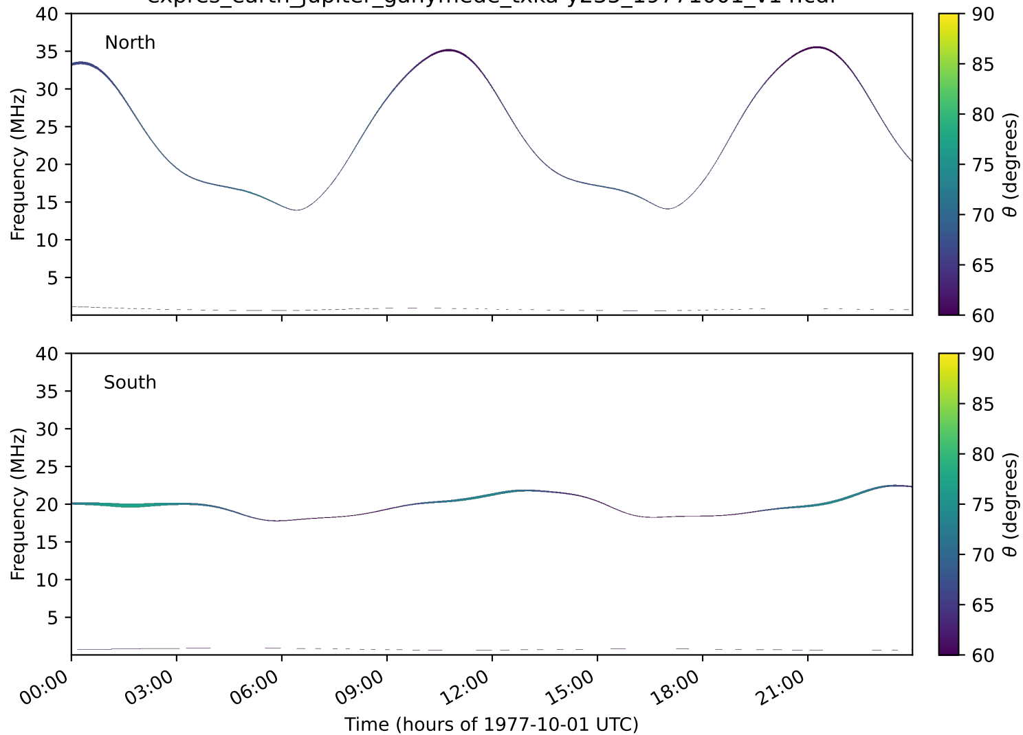
expres_earth_jupiter_ganymede_txka-y235_19771001_v14.cdf
