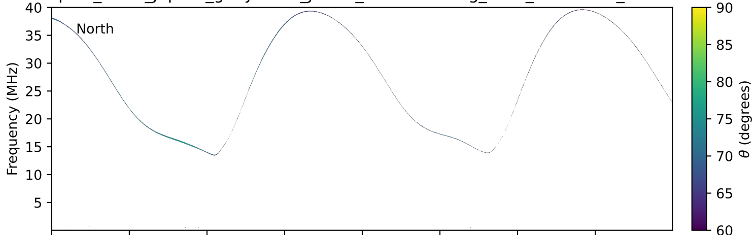
expres_earth_jupiter_ganymede_jrm09_lossc-wid1deg_3kev_19771001_v11.cdf
