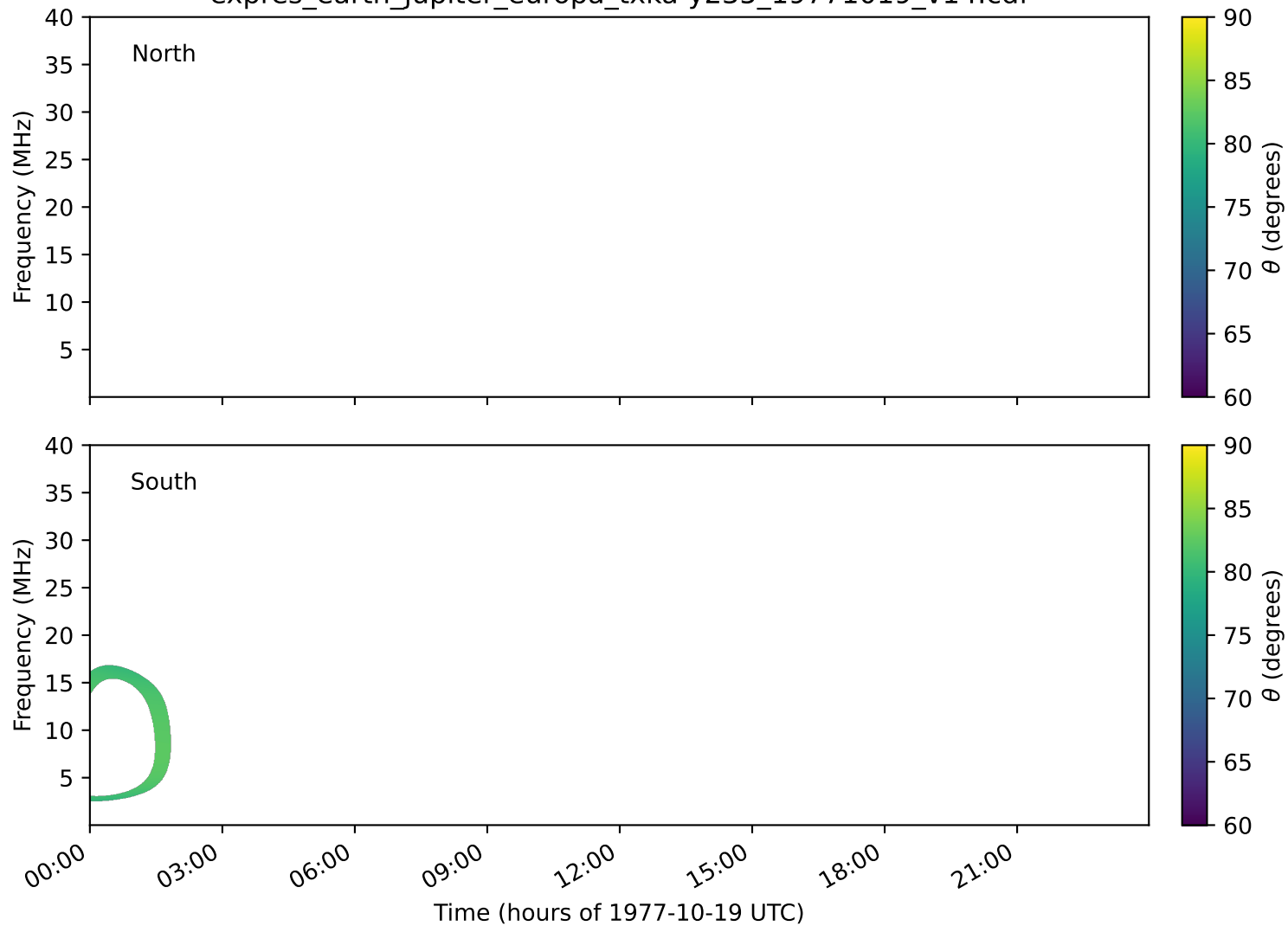
expres_earth_jupiter_europa_txka-y235_19771019_v14.cdf
