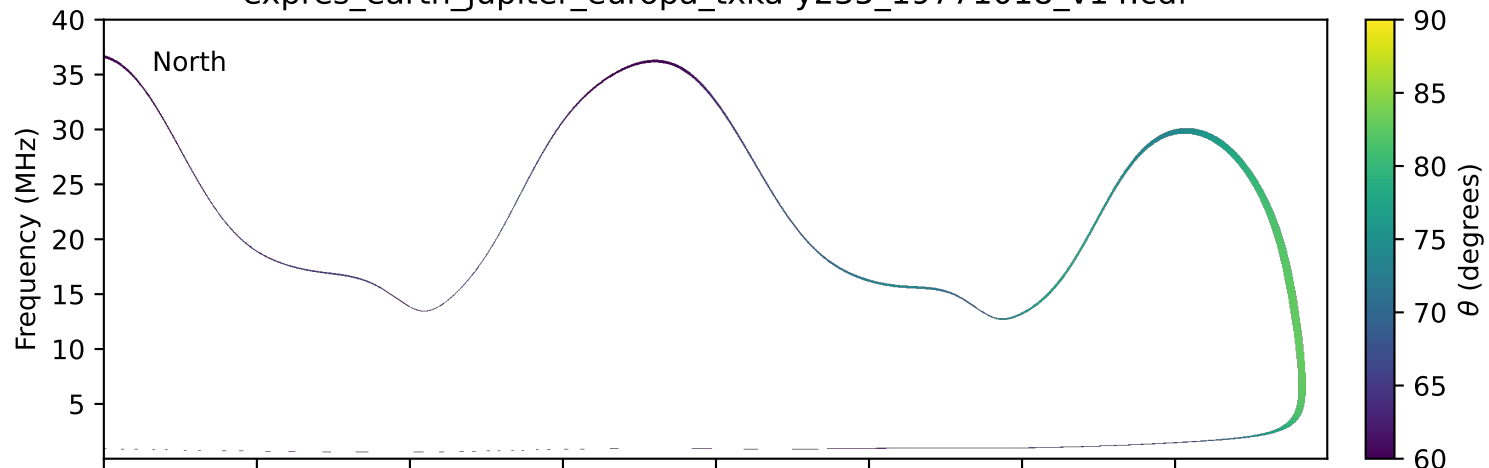
expres_earth_jupiter_europa_txka-y235_19771018_v14.cdf
