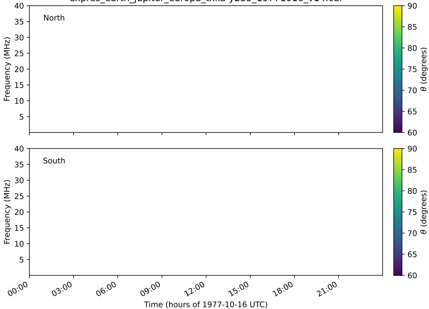
expres_earth_jupiter_europa_txka-y235_19771016_v14.cdf
