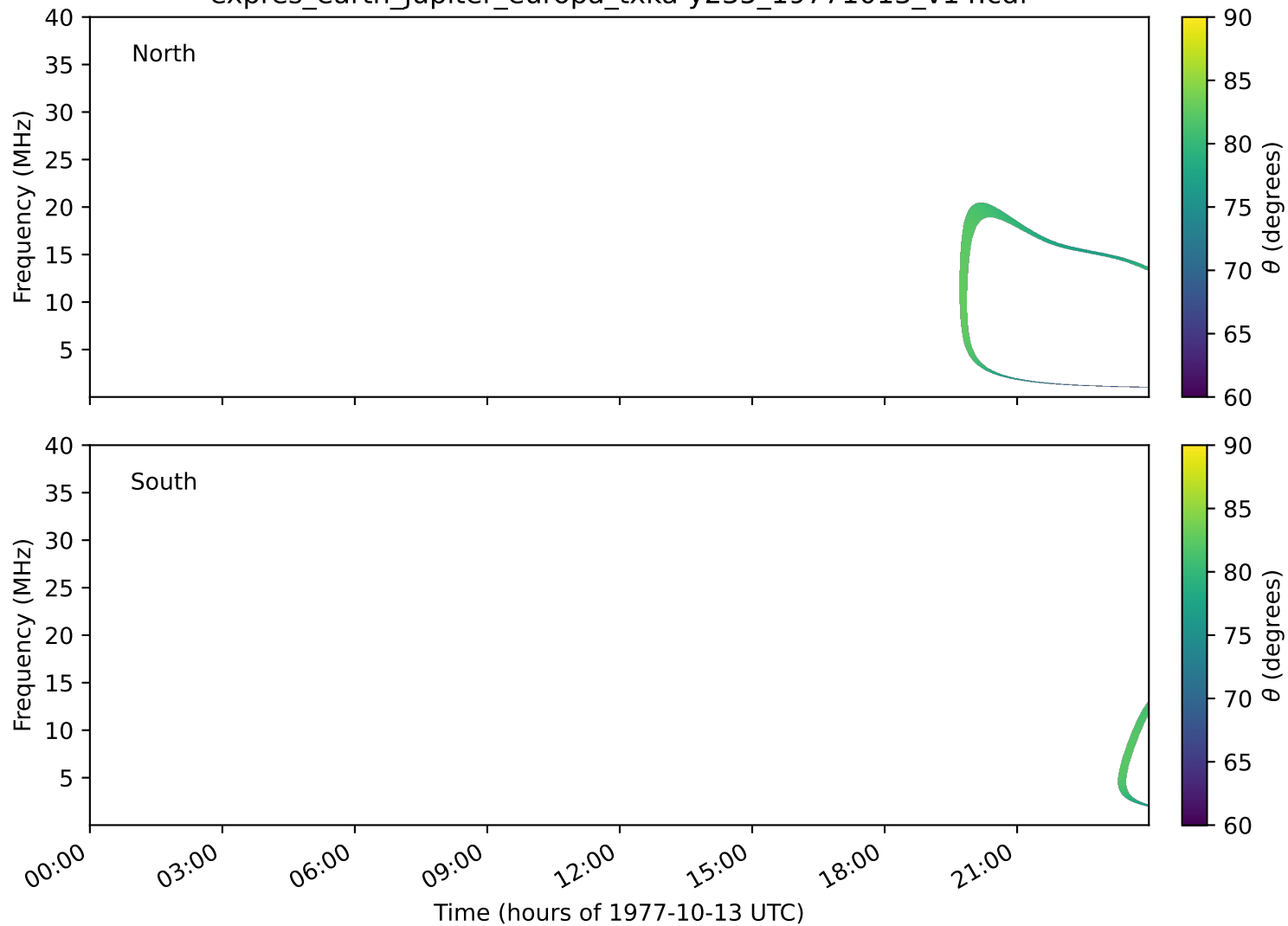
expres_earth_jupiter_europa_txka-y235_19771013_v14.cdf
