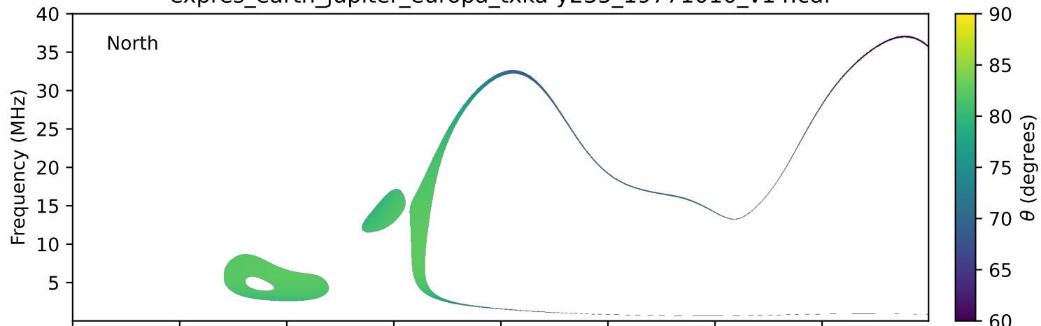
expres_earth_jupiter_europa_txka-y235_19771010_v14.cdf
