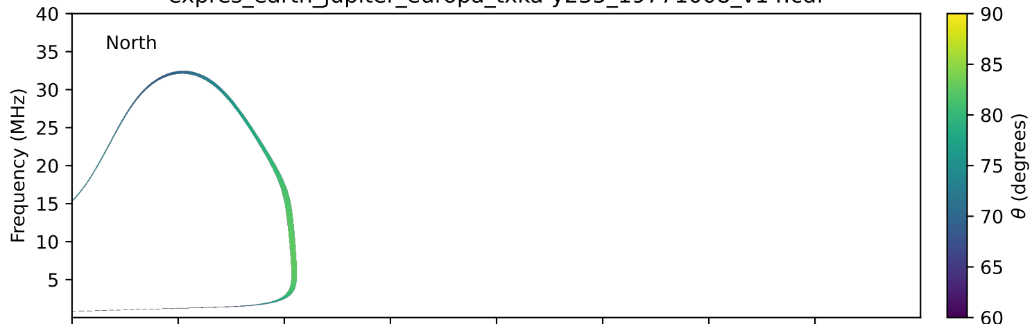
expres_earth_jupiter_europa_txka-y235_19771008_v14.cdf
