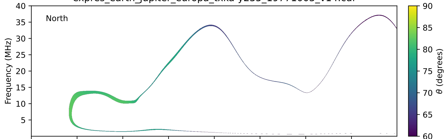
expres_earth_jupiter_europa_txka-y235_19771003_v14.cdf
