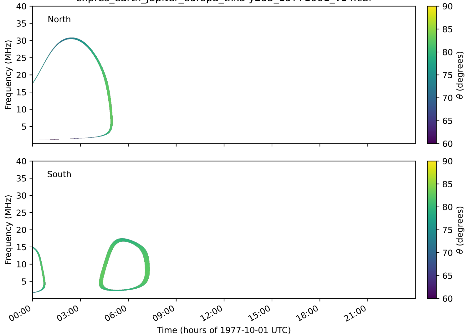
expres_earth_jupiter_europa_txka-y235_19771001_v14.cdf
