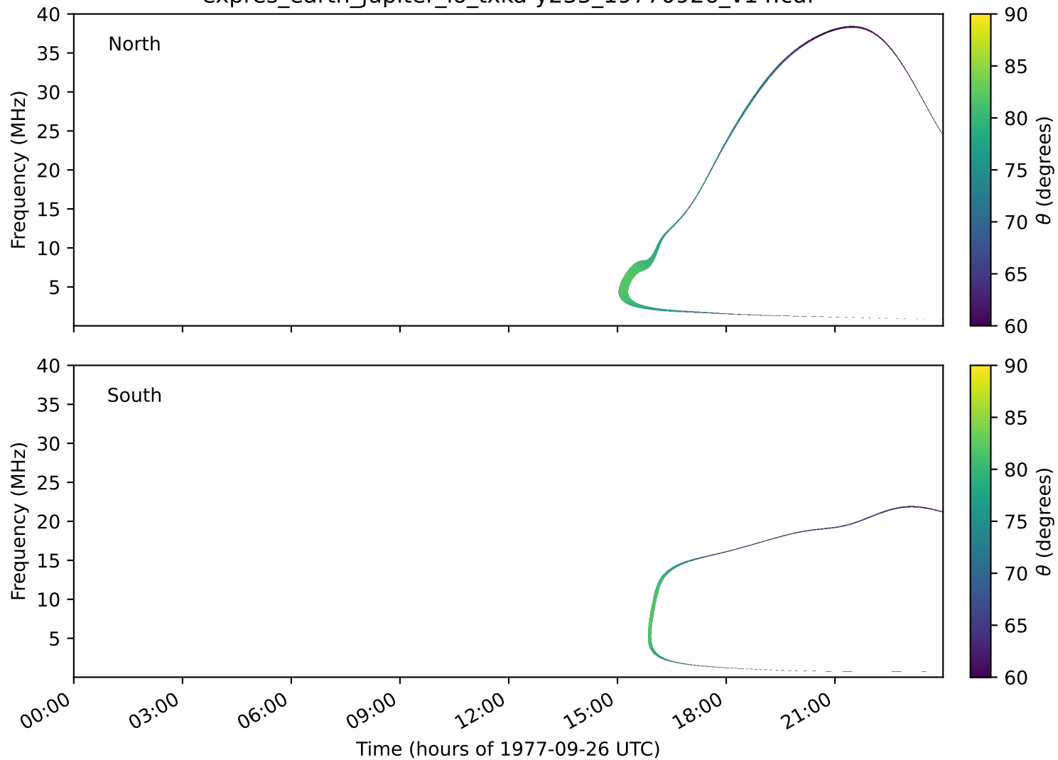
expres_earth_jupiter_io_txka-y235_19770926_v14.cdf
