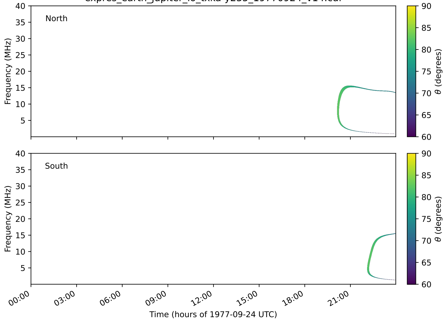
expres_earth_jupiter_io_txka-y235_19770924_v14.cdf
