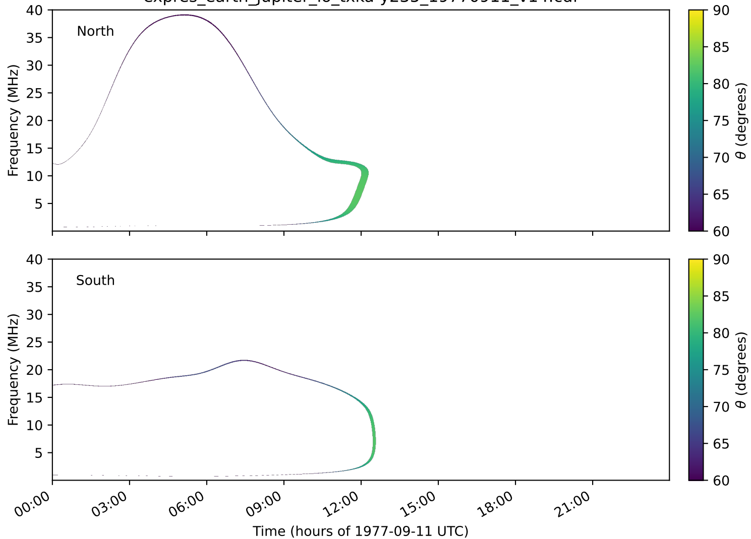
expres_earth_jupiter_io_txka-y235_19770911_v14.cdf
