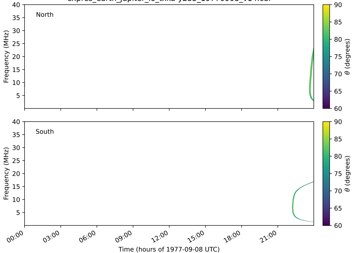
expres_earth_jupiter_io_txka-y235_19770908_v14.cdf
