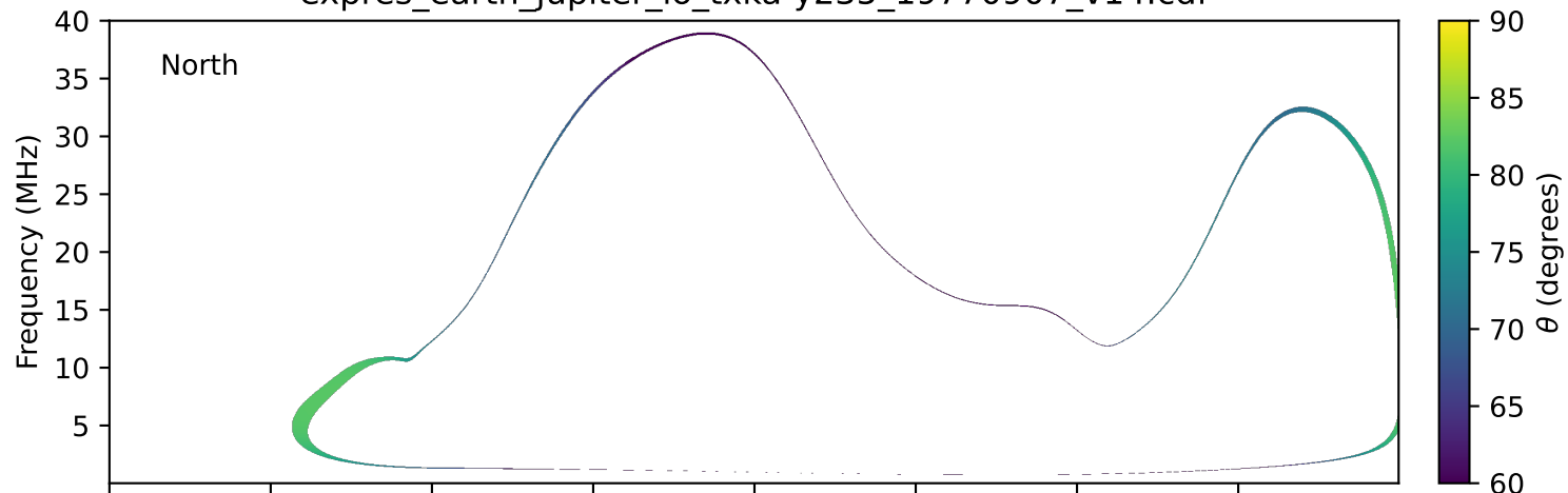
expres_earth_jupiter_io_txka-y235_19770907_v14.cdf
