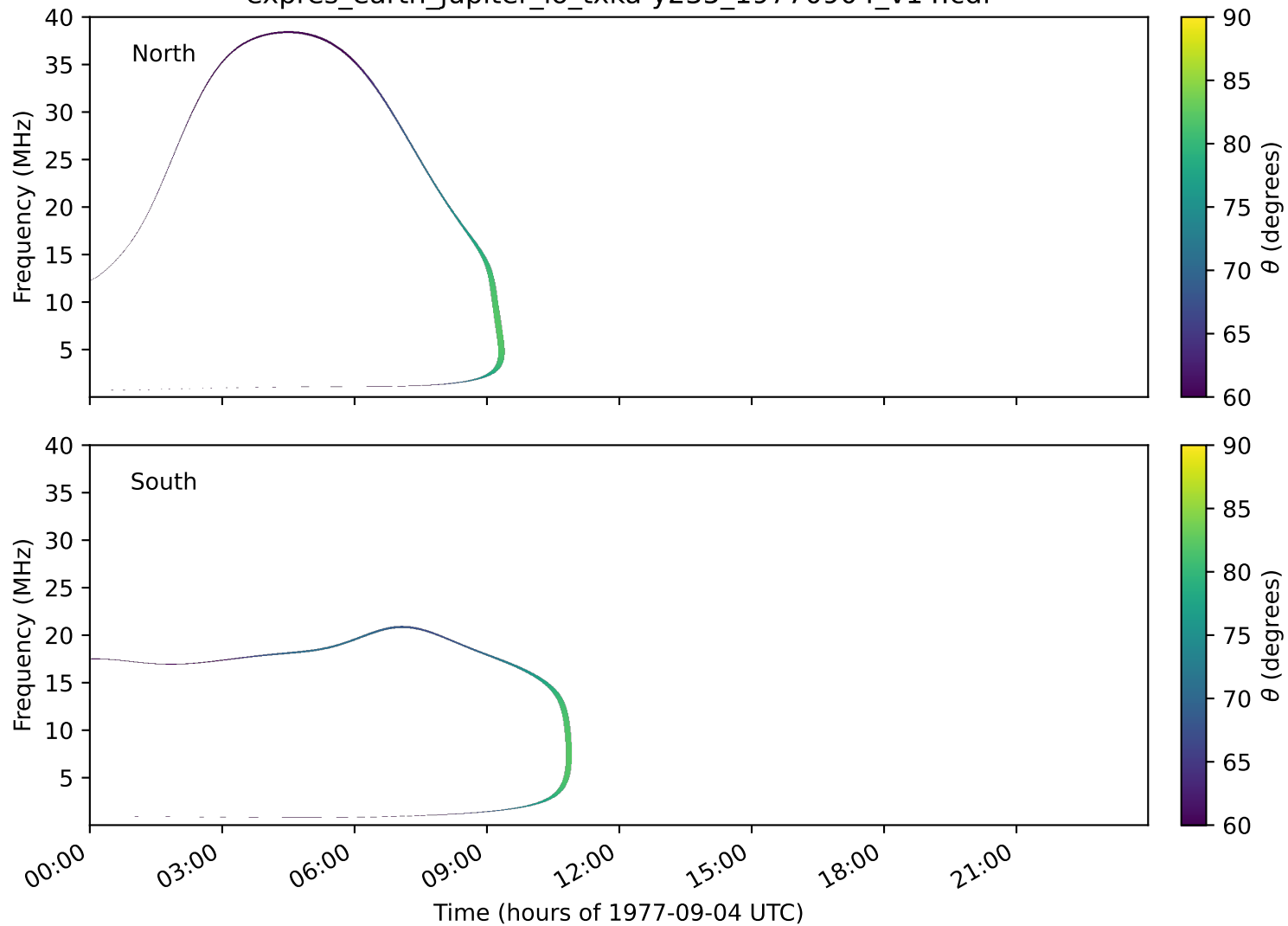
expres_earth_jupiter_io_txka-y235_19770904_v14.cdf
