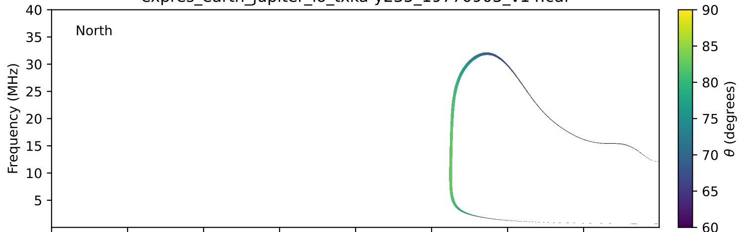
expres_earth_jupiter_io_txka-y235_19770903_v14.cdf
