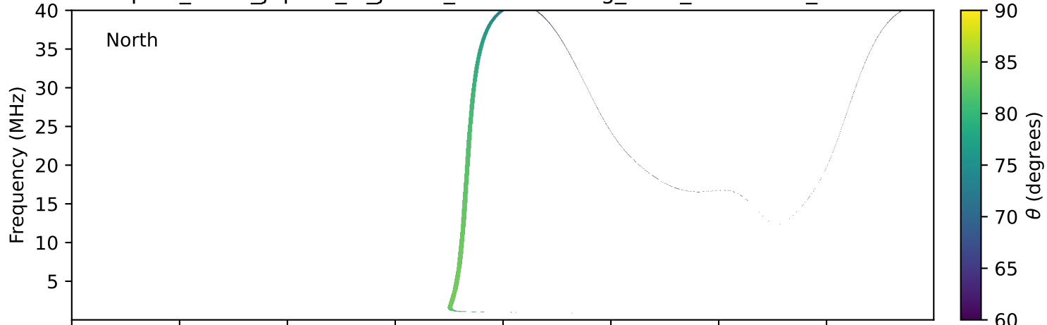
expres_earth_jupiter_io_jrm33_lossc-wid1deg_3kev_19770928_v11.cdf
