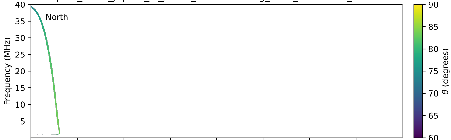
expres_earth_jupiter_io_jrm33_lossc-wid1deg_3kev_19770915_v11.cdf
