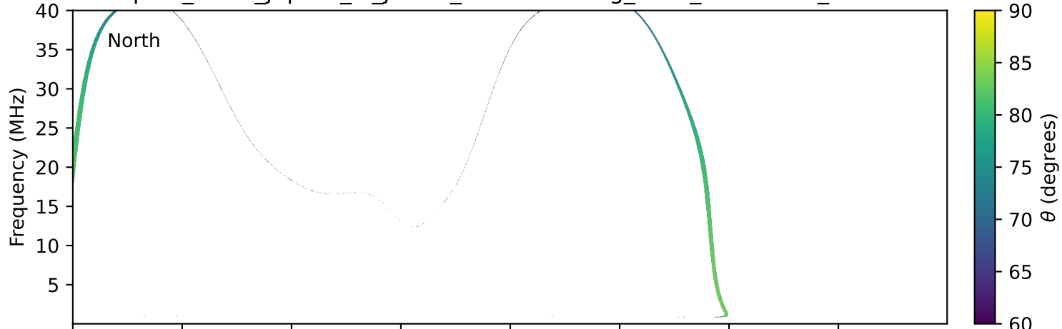
expres_earth_jupiter_io_jrm33_lossc-wid1deg_3kev_19770909_v11.cdf
